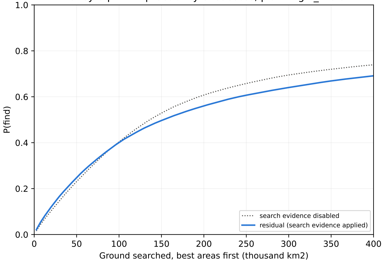
Davey eq. 11.2: probability of success, planning P_D 0.9
